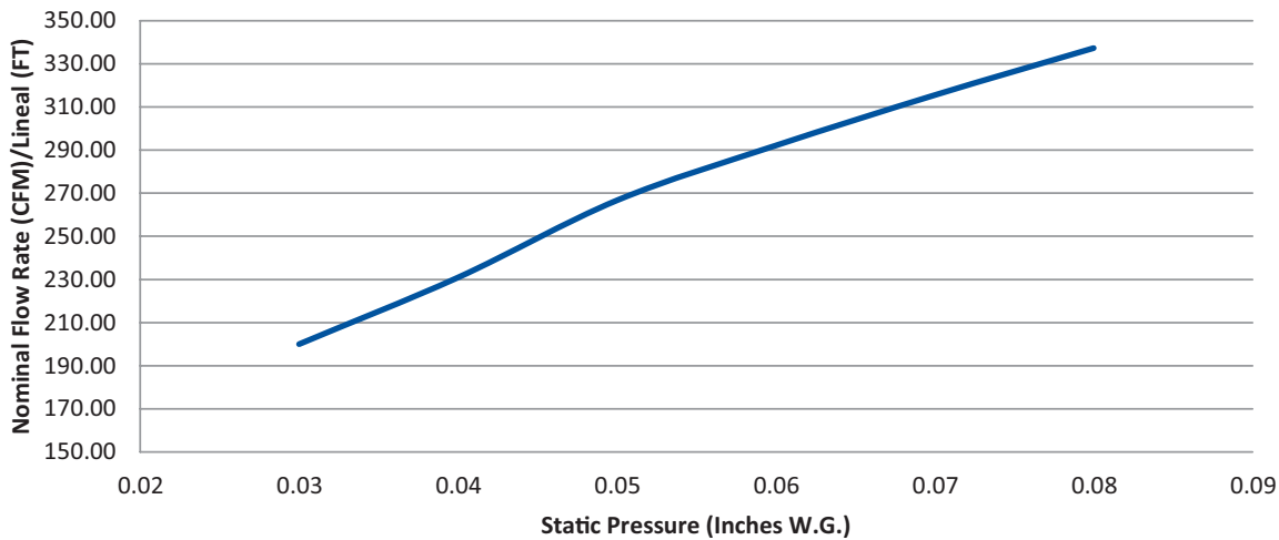
Air Flow Performance Per Lineal Foot Based on 8" (203mm) Wide Grille
