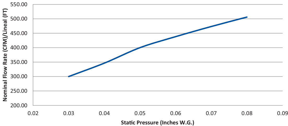
Air Flow Performance Per Lineal Foot Based on 12" (305mm) Wide Grille
