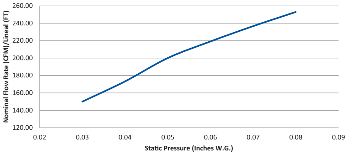
Air Flow Performance Per Lineal Foot Based on 6" (152mm) Wide Grille
