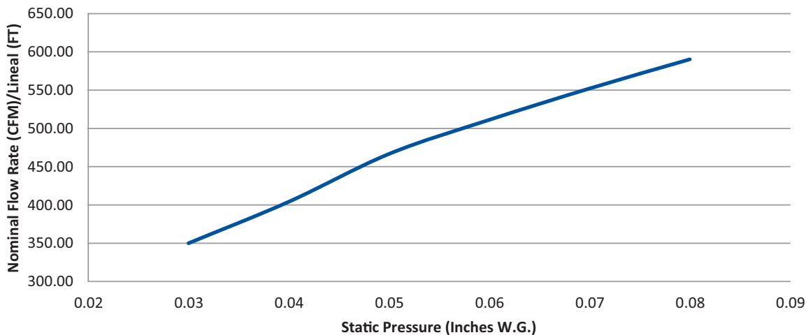
Air Flow Performance Per Lineal Foot Based on 14" (356mm) Wide Grille
