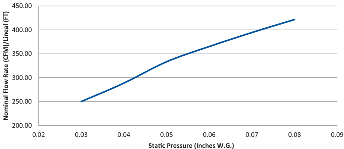
Air Flow Performance Per Lineal Foot Based on 10" (254mm) Wide Grille
