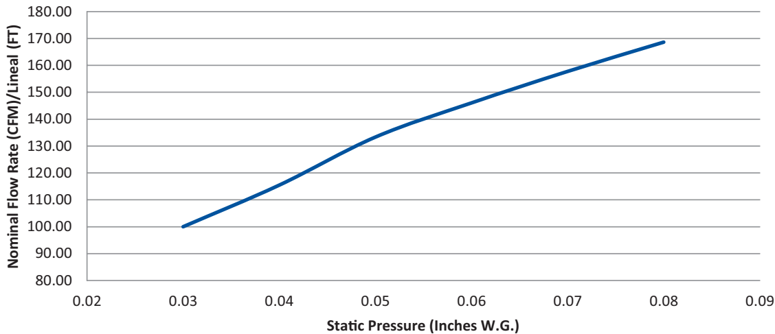
Air Flow Performance Per Lineal Foot Based on 4" (102mm) Wide Grille
