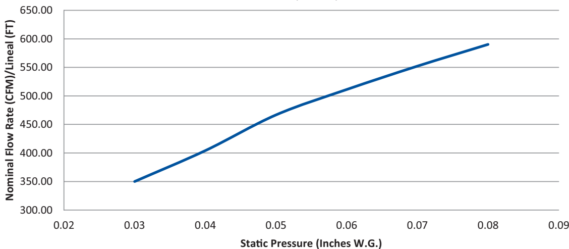
Air Flow Performance Per Lineal Foot Based on 16" (406mm) Wide Grille
